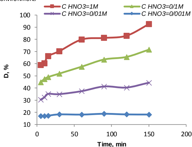
Fig. 7. Desorption for Ag ions by PLA adsorbent; conditions: initial \text{Ag}^+ concentration=1g/L, pH= 7 and temperature=25 °C.
